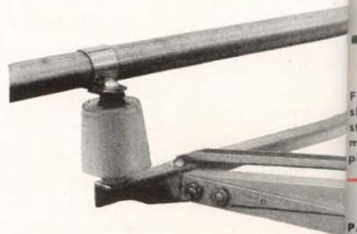
Fig. 7. Side detail view at the corner of the frame looking from the right side of the boom, showing part 1 and 2 attached to the element truss.
