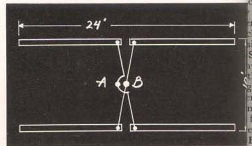
Fig. 2. Schematic diagram of the DIRECTIONNULL antenna showing over-all dimensions, phasing line and feedline "A" and "B."
