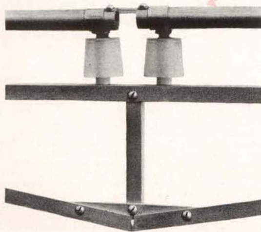
Fig. 6. Detail view at the center of the element support trusses. The element sections are spaced \frac{1}{4} inches and the phasing line is fastened to the tubing with a spacing of 2 inches between hole centers.
