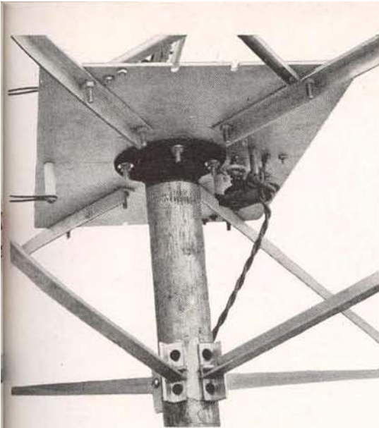
Fig. 8. Bottom view of the aluminum mounting plate showing the braces attached to the pipe mast and matching stub insulator. The clock motor that drives the capacitor is mounted on metal pillars 3 inches from the center of the plate.
